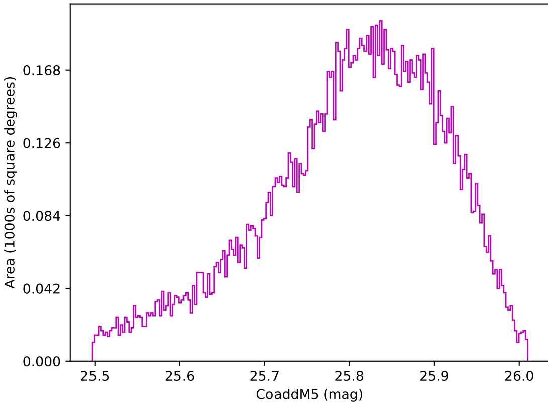
too_elab_r32_d3_giz_v3.4_10yrs WFD z band: CoaddM5
