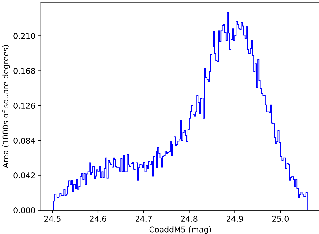
too_elab_r32_d3_giz_v3.4_10yrs WFD y band: CoaddM5
