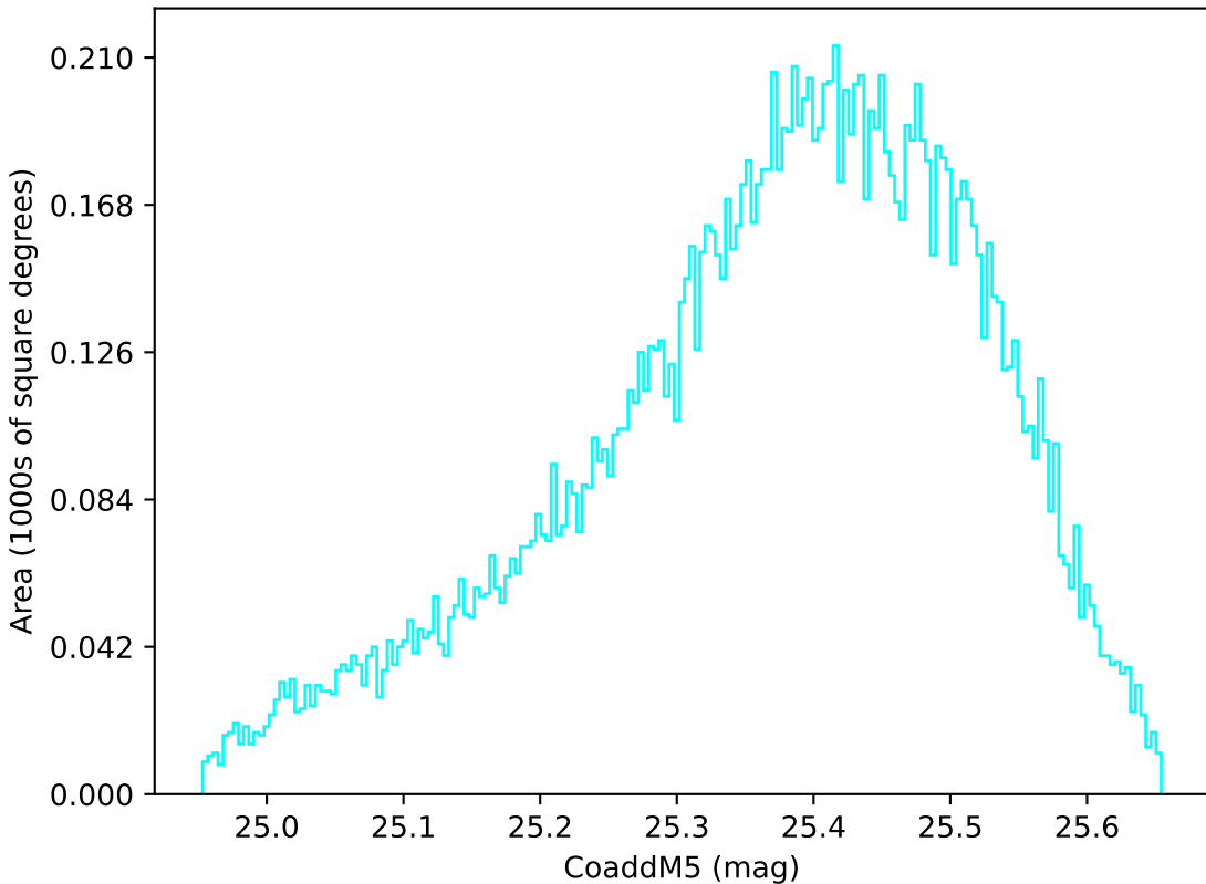
too_elab_r32_d3_giz_v3.4_10yrs WFD u band: CoaddM5
