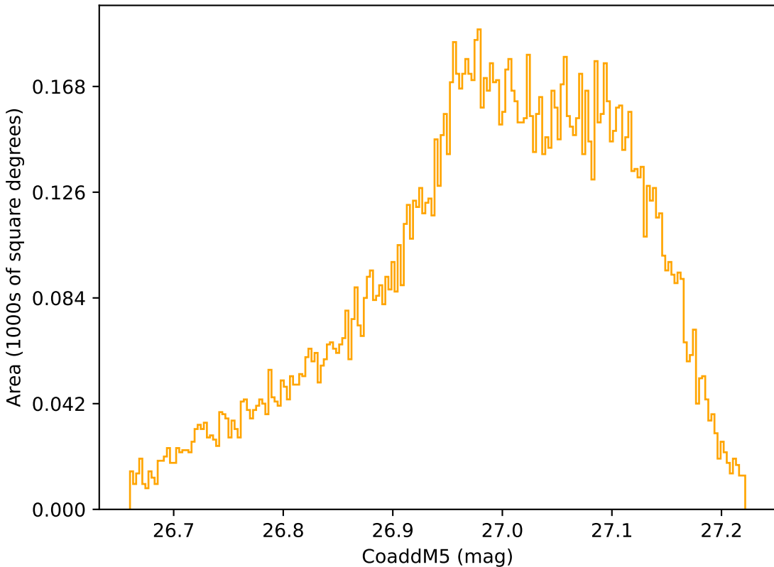
too_elab_r32_d3_giz_v3.4_10yrs WFD r band: CoaddM5
