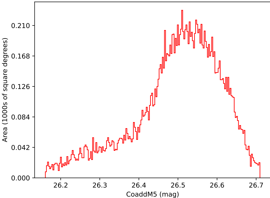
too_elab_r32_d3_giz_v3.4_10yrs WFD i band: CoaddM5
