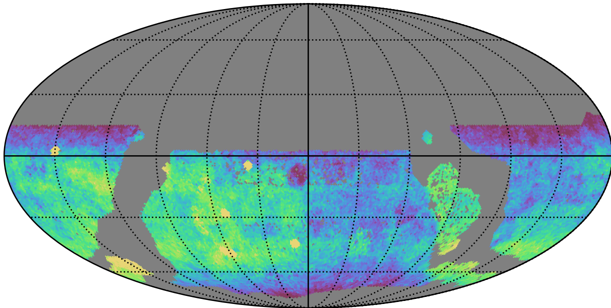
too_elab_r32_d3_giz_v3.4_10yrs WFD g band: CoaddM5
