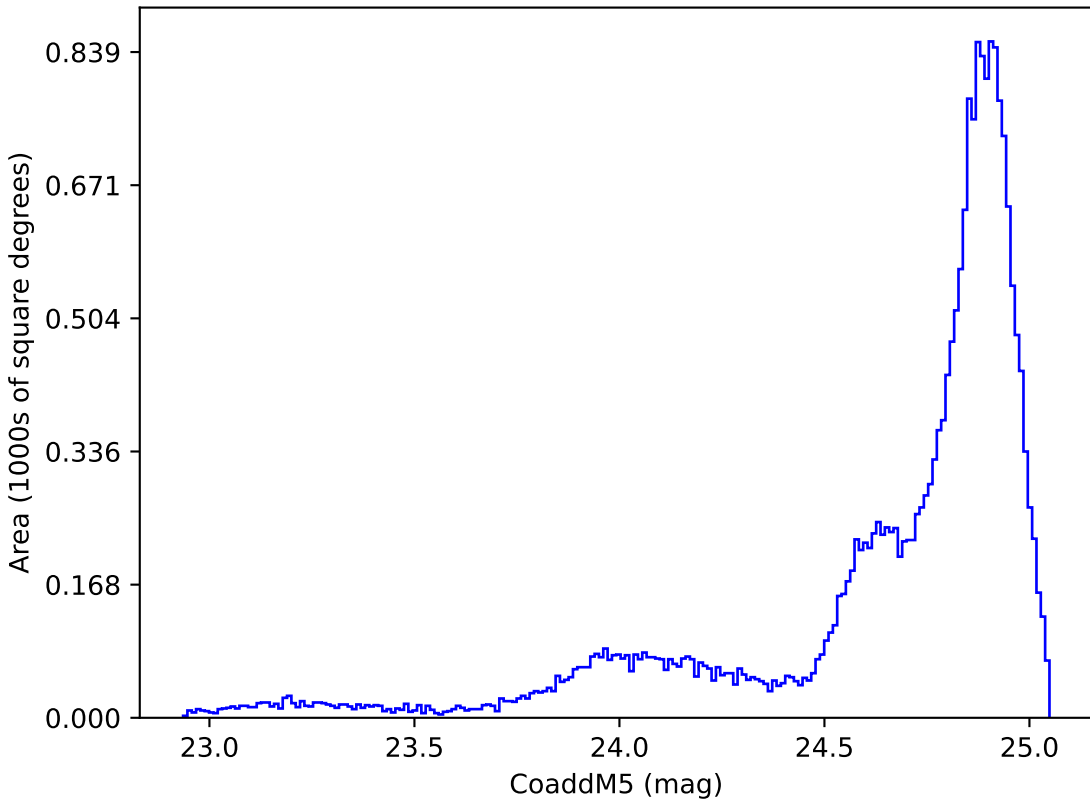
too_elab_r32_d3_giz_v3.4_10yrs All sky y band: CoaddM5
