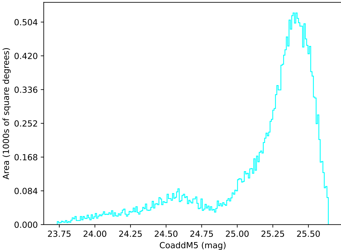
too_elab_r32_d3_giz_v3.4_10yrs All sky u band: CoaddM5
