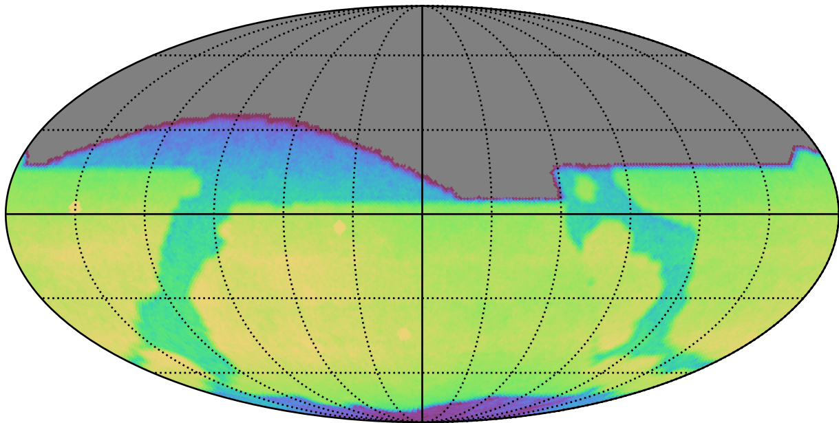
too_elab_r32_d3_giz_v3.4_10yrs All sky r band: CoaddM5
