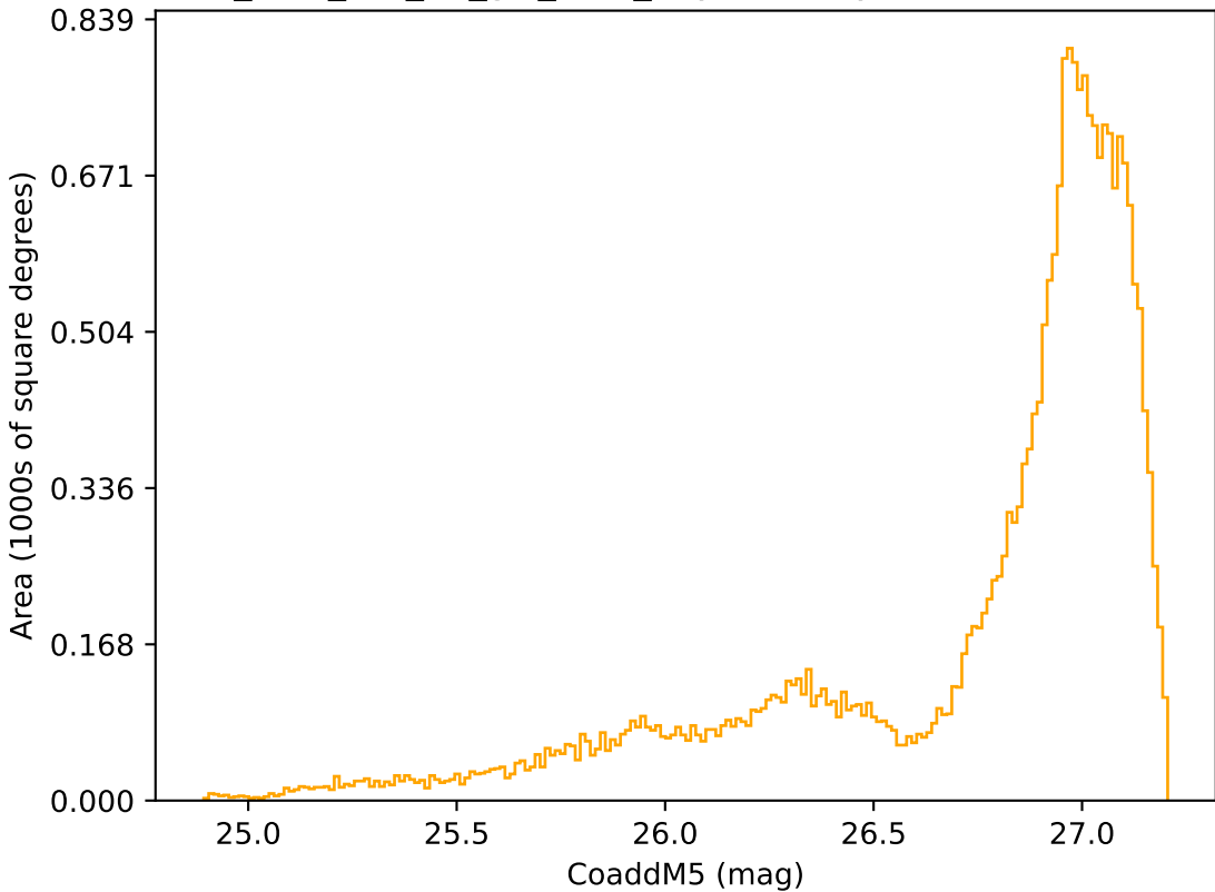
too_elab_r32_d3_giz_v3.4_10yrs All sky r band: CoaddM5
