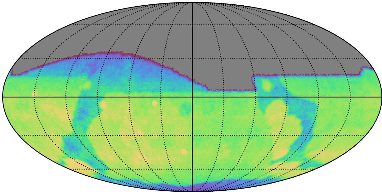
too_elab_r32_d3_giz_v3.4_10yrs All sky g band: CoaddM5
