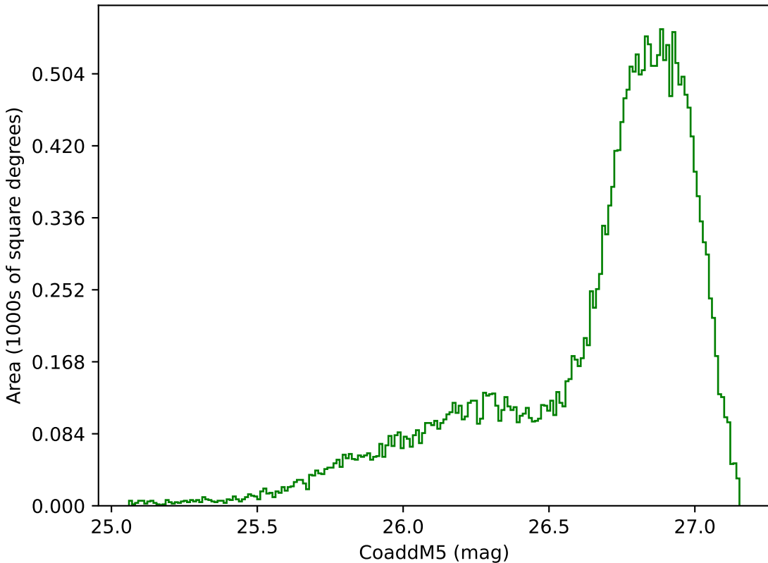
too_elab_r32_d3_giz_v3.4_10yrs All sky g band: CoaddM5
