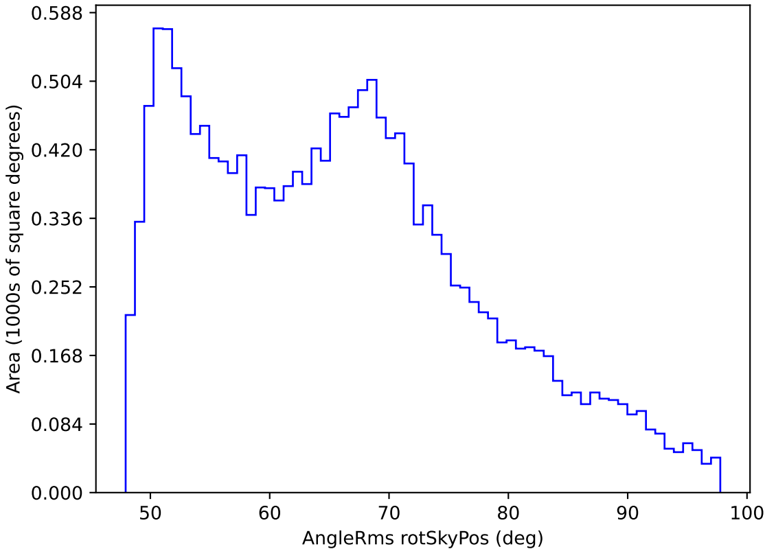
too_elab_r32_d3_giz_v3.4_10yrs WFD r band: AngleRms rotSkyPos
