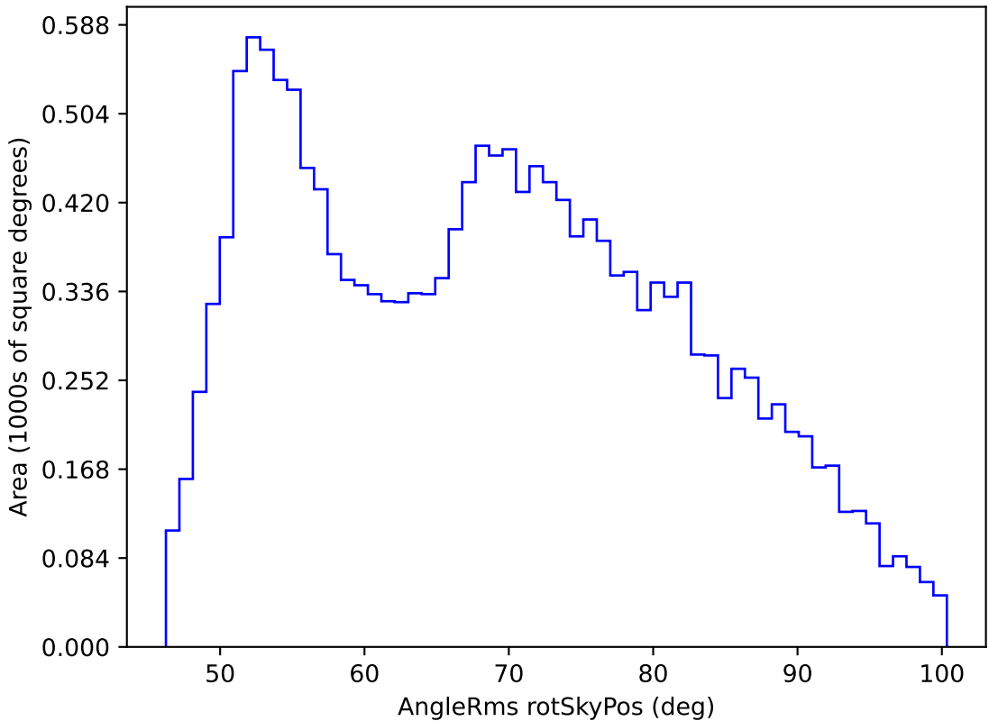
too_elab_r32_d3_giz_v3.4_10yrs WFD g band: AngleRms rotSkyPos
