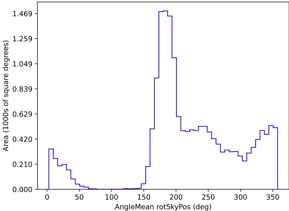
too_elab_r32_d3_giz_v3.4_10yrs WFD u band: AngleMean rotSkyPos
