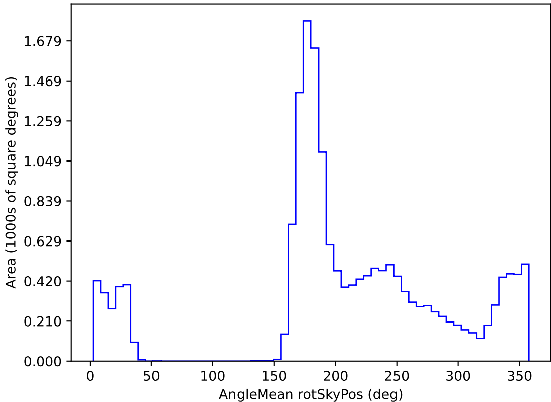
too_elab_r32_d3_giz_v3.4_10yrs WFD r band: AngleMean rotSkyPos
