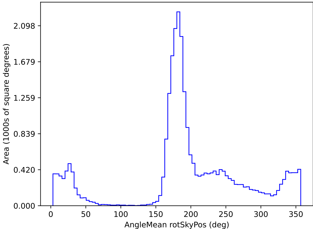
too_elab_r32_d3_giz_v3.4_10yrs All sky r band: AngleMean rotSkyPos
