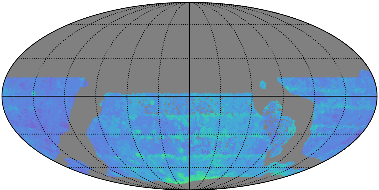
too_elab_r32_d3_giz_v3.4_10yrs WFD y band: 80thPercentile Season Length
