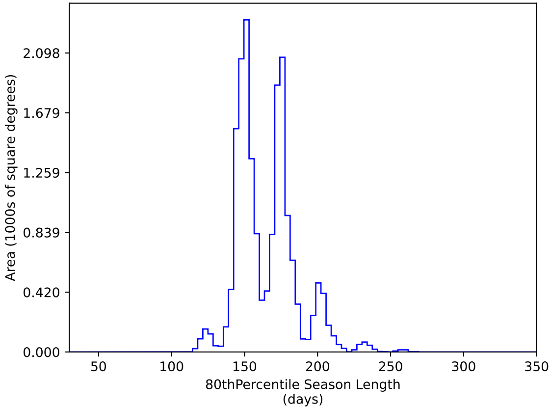
too_elab_r32_d3_giz_v3.4_10yrs WFD y band: 80thPercentile Season Length
