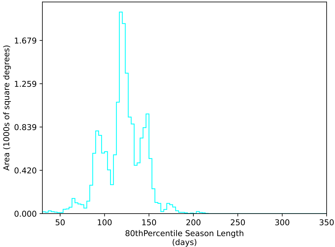
too_elab_r32_d3_giz_v3.4_10yrs WFD u band: 80thPercentile Season Length
