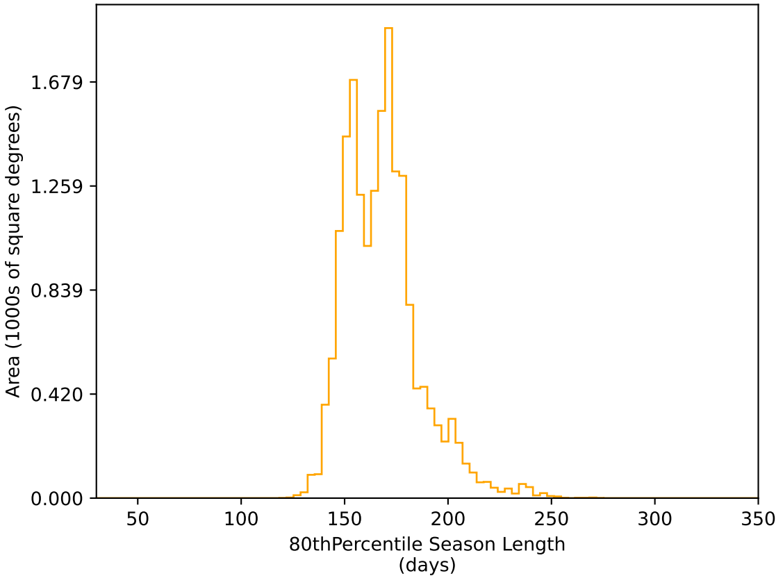
too_elab_r32_d3_giz_v3.4_10yrs WFD r band: 80thPercentile Season Length
