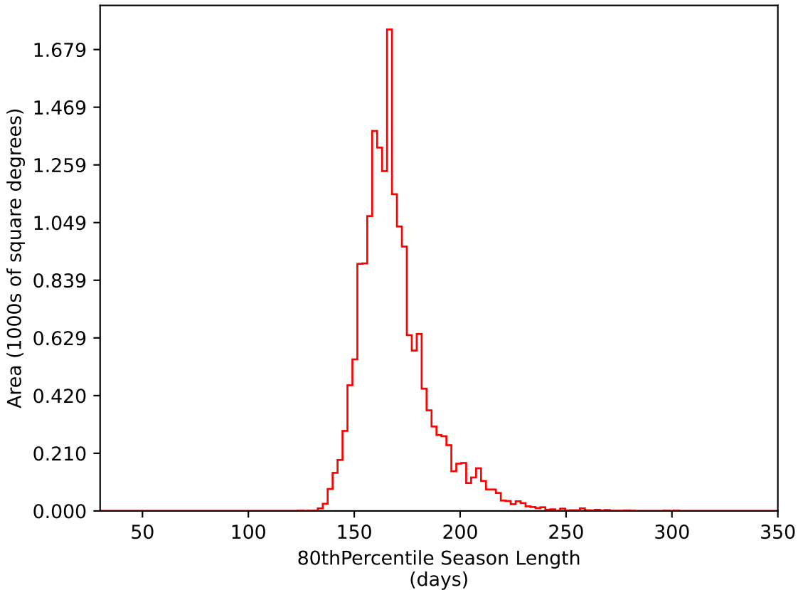
too_elab_r32_d3_giz_v3.4_10yrs WFD i band: 80thPercentile Season Length
