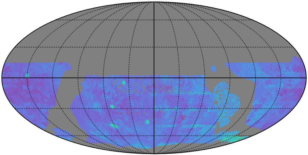
too_elab_r32_d3_giz_v3.4_10yrs WFD g band: 80thPercentile Season Length
