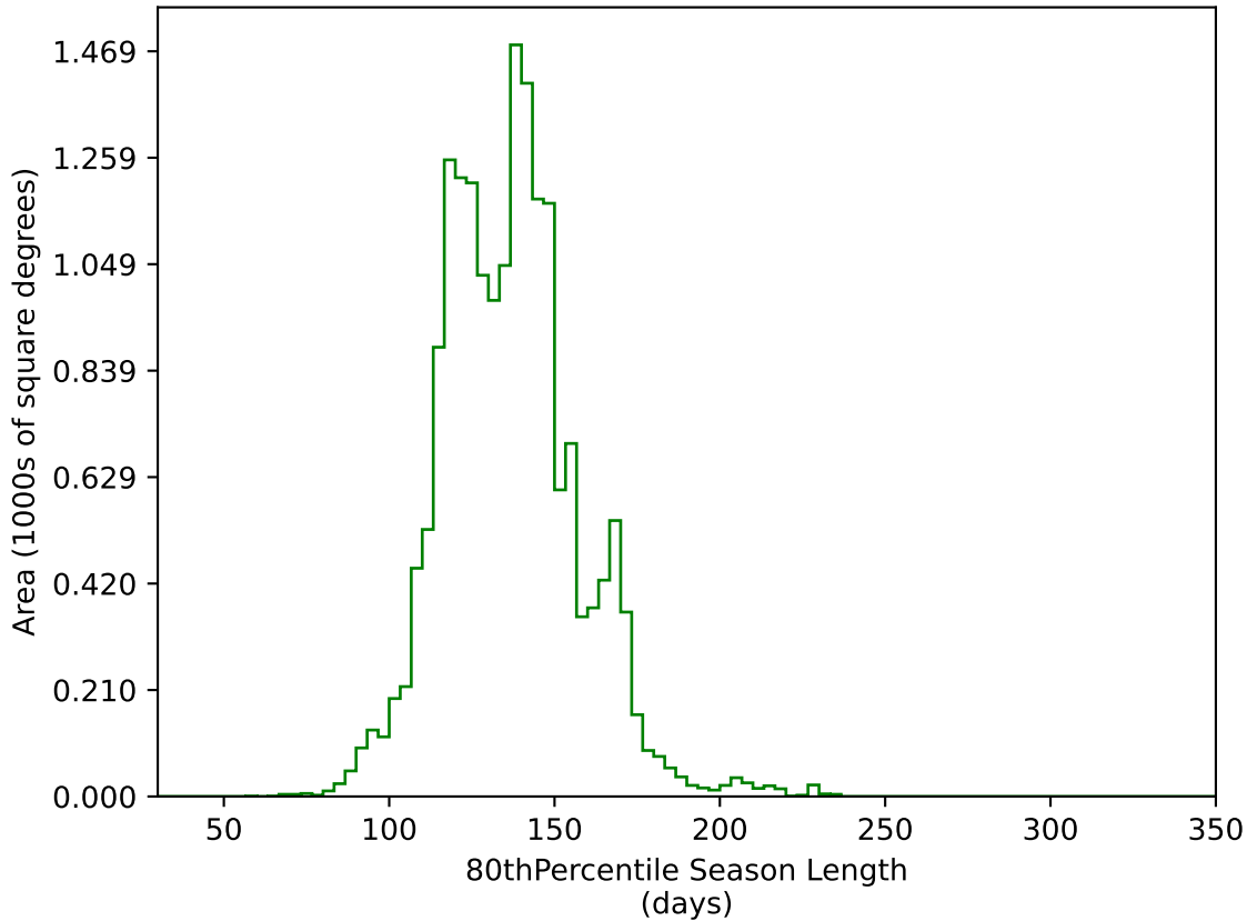
too_elab_r32_d3_giz_v3.4_10yrs WFD g band: 80thPercentile Season Length
