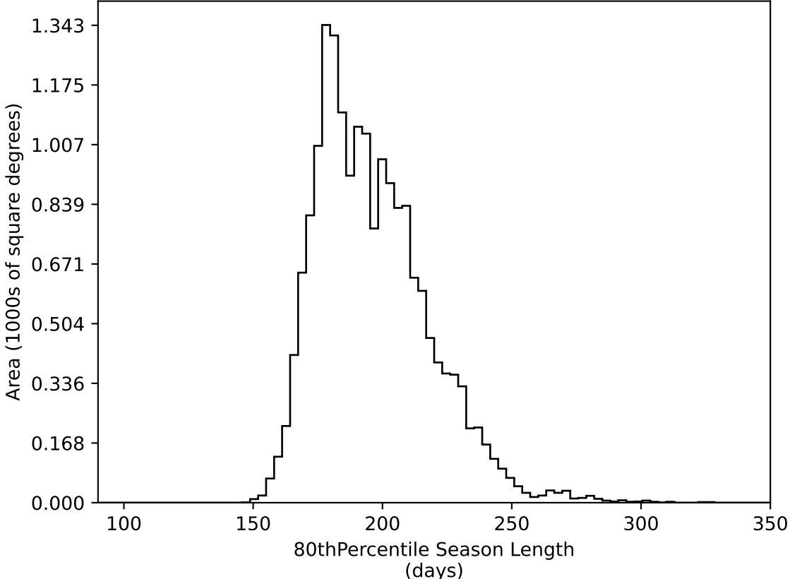
too_elab_r32_d3_giz_v3.4_10yrs WFD all bands: 80thPercentile Season Length
