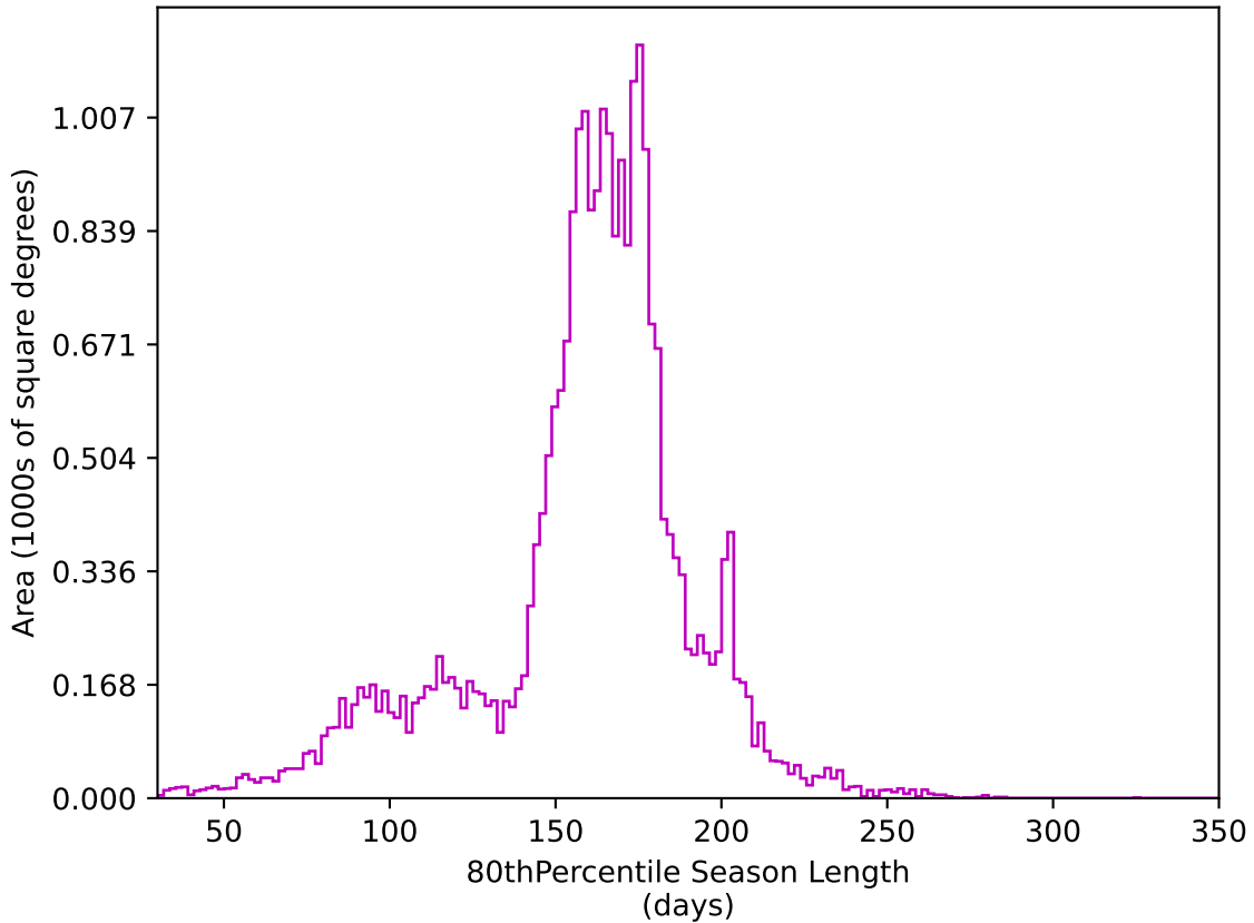
too_elab_r32_d3_giz_v3.4_10yrs All sky z band: 80thPercentile Season Length
