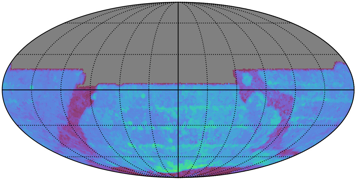
too_elab_r32_d3_giz_v3.4_10yrs All sky y band: 80thPercentile Season Length
