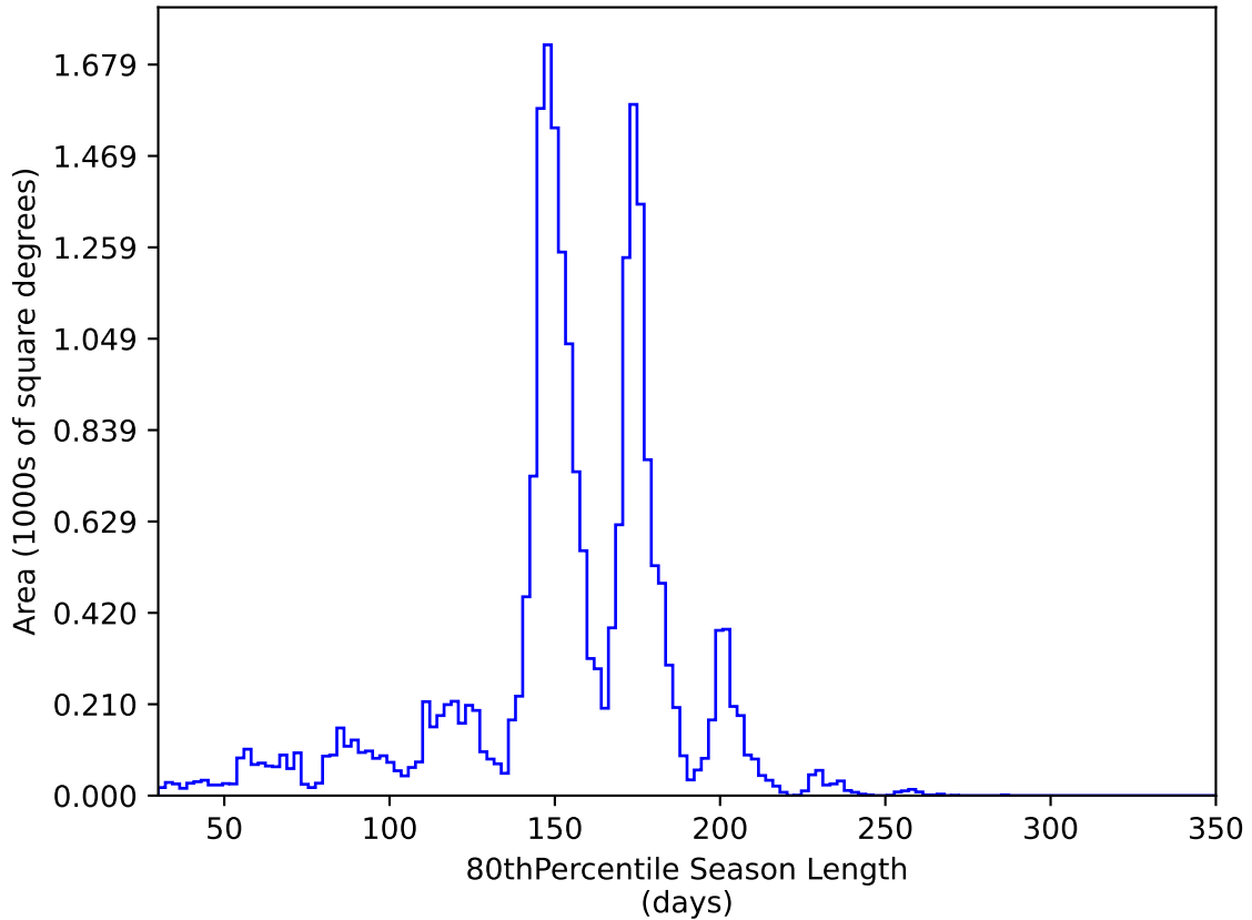
too_elab_r32_d3_giz_v3.4_10yrs All sky y band: 80thPercentile Season Length
