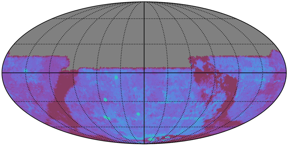
too_elab_r32_d3_giz_v3.4_10yrs All sky u band: 80thPercentile Season Length
