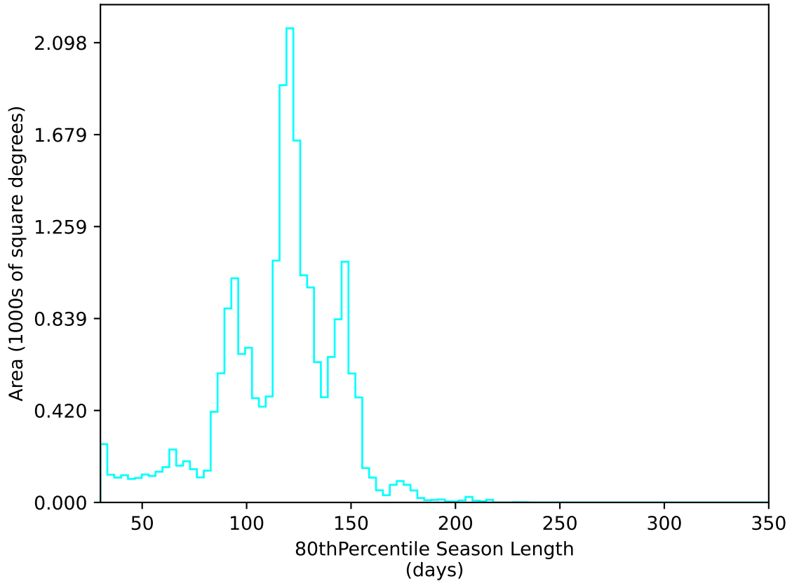
too_elab_r32_d3_giz_v3.4_10yrs All sky u band: 80thPercentile Season Length
