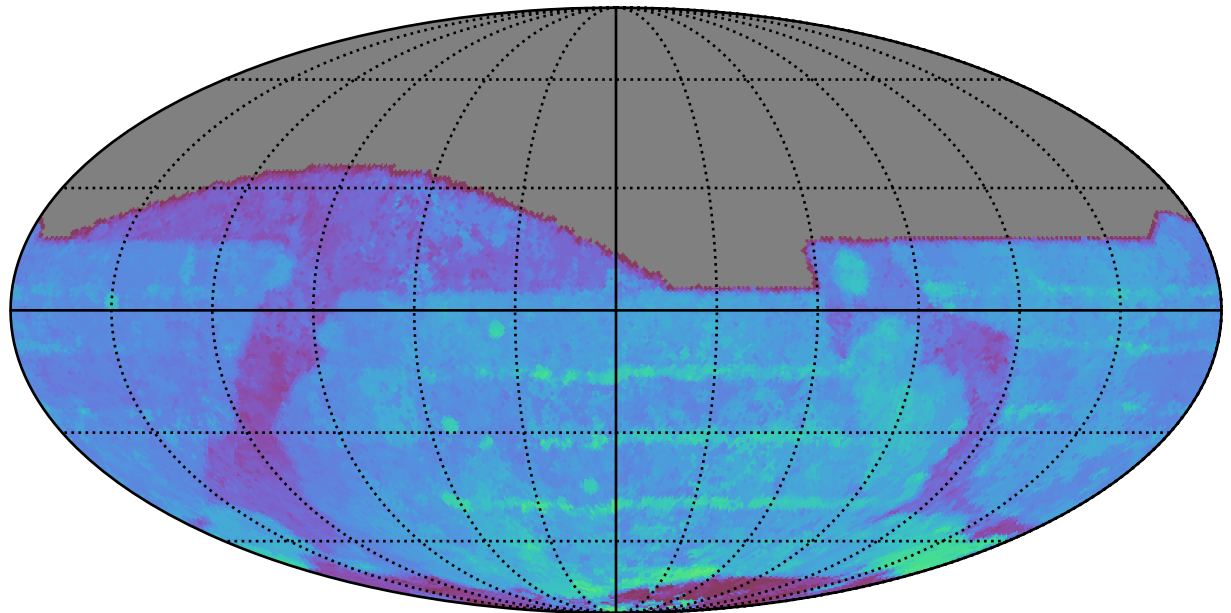
too_elab_r32_d3_giz_v3.4_10yrs All sky r band: 80thPercentile Season Length
