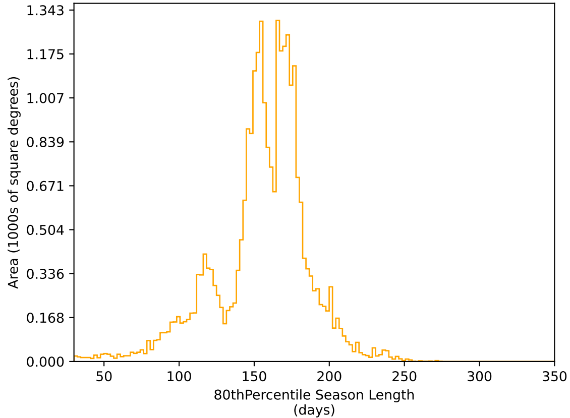
too_elab_r32_d3_giz_v3.4_10yrs All sky r band: 80thPercentile Season Length
