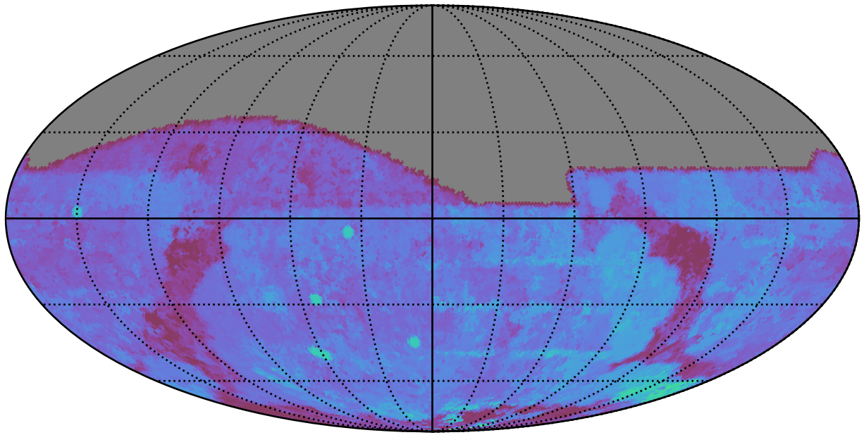
too_elab_r32_d3_giz_v3.4_10yrs All sky g band: 80thPercentile Season Length
