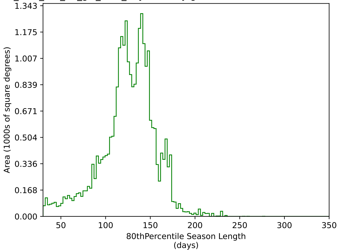
too_elab_r32_d3_giz_v3.4_10yrs All sky g band: 80thPercentile Season Length
