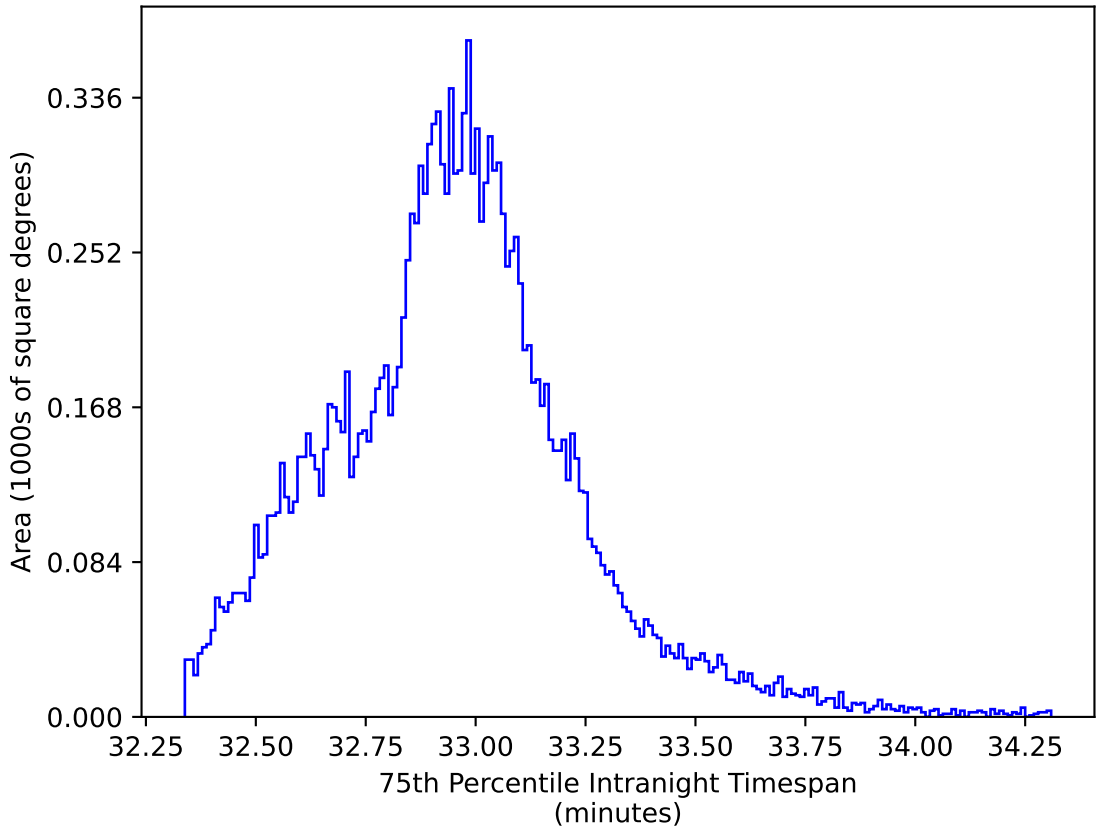
too_elab_r32_d3_giz_v3.4_10yrs WFD y band: 75th Percentile Intranight Timespan
