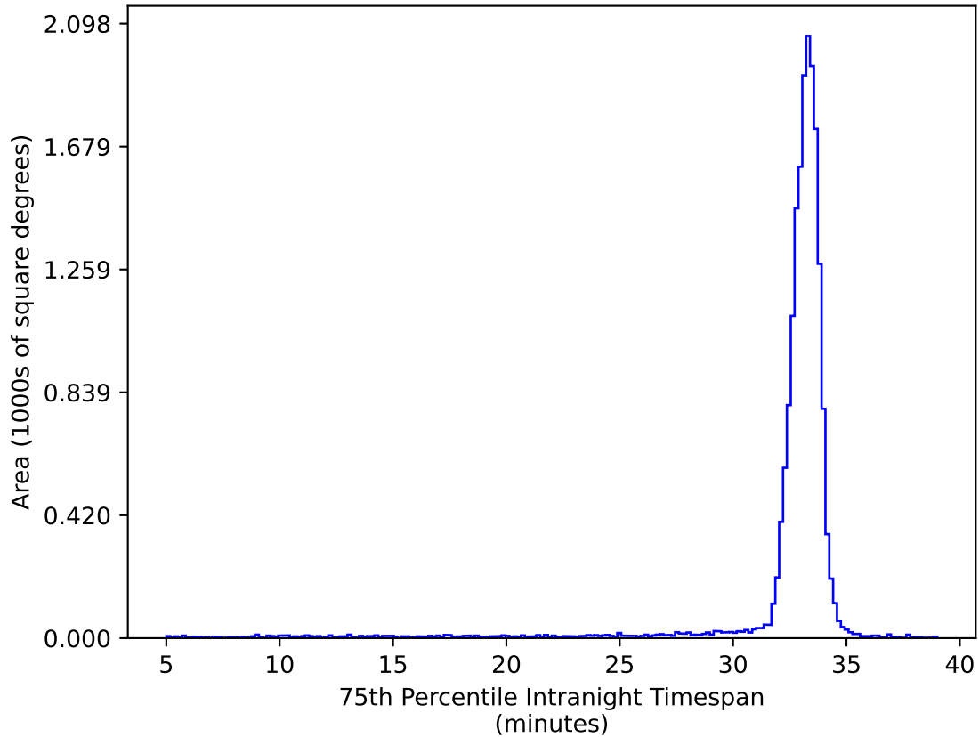
too_elab_r32_d3_giz_v3.4_10yrs WFD ug bands: 75th Percentile Intranight Timespan
