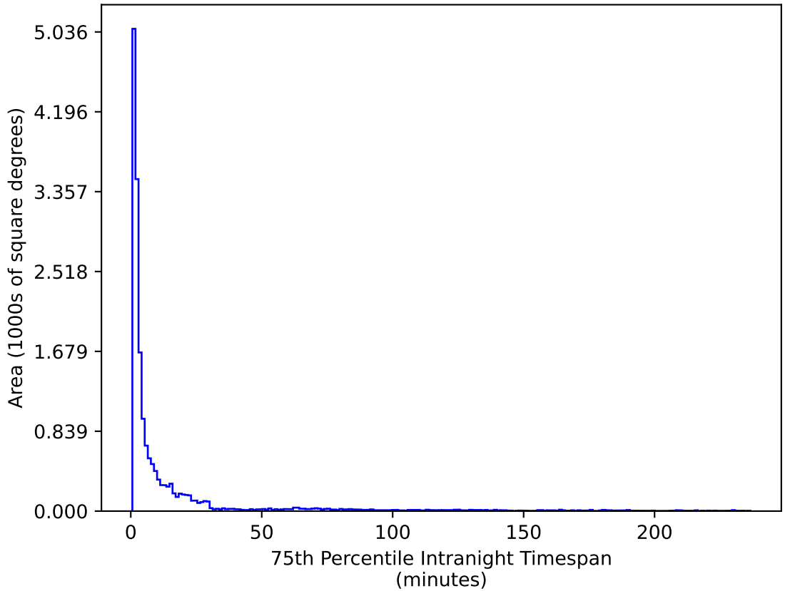
too_elab_r32_d3_giz_v3.4_10yrs WFD u band: 75th Percentile Intranight Timespan
