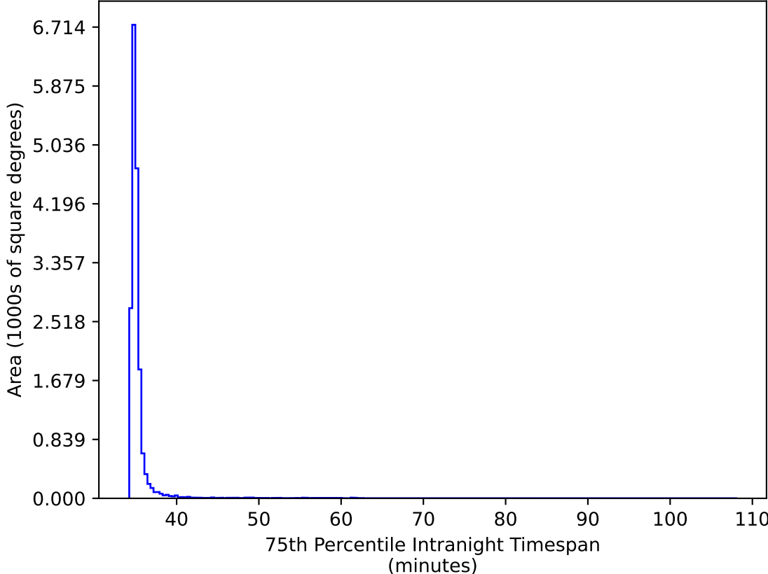
too_elab_r32_d3_giz_v3.4_10yrs WFD gr bands: 75th Percentile Intranight Timespan
