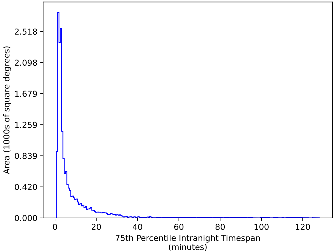
too_elab_r32_d3_giz_v3.4_10yrs WFD g band: 75th Percentile Intranight Timespan
