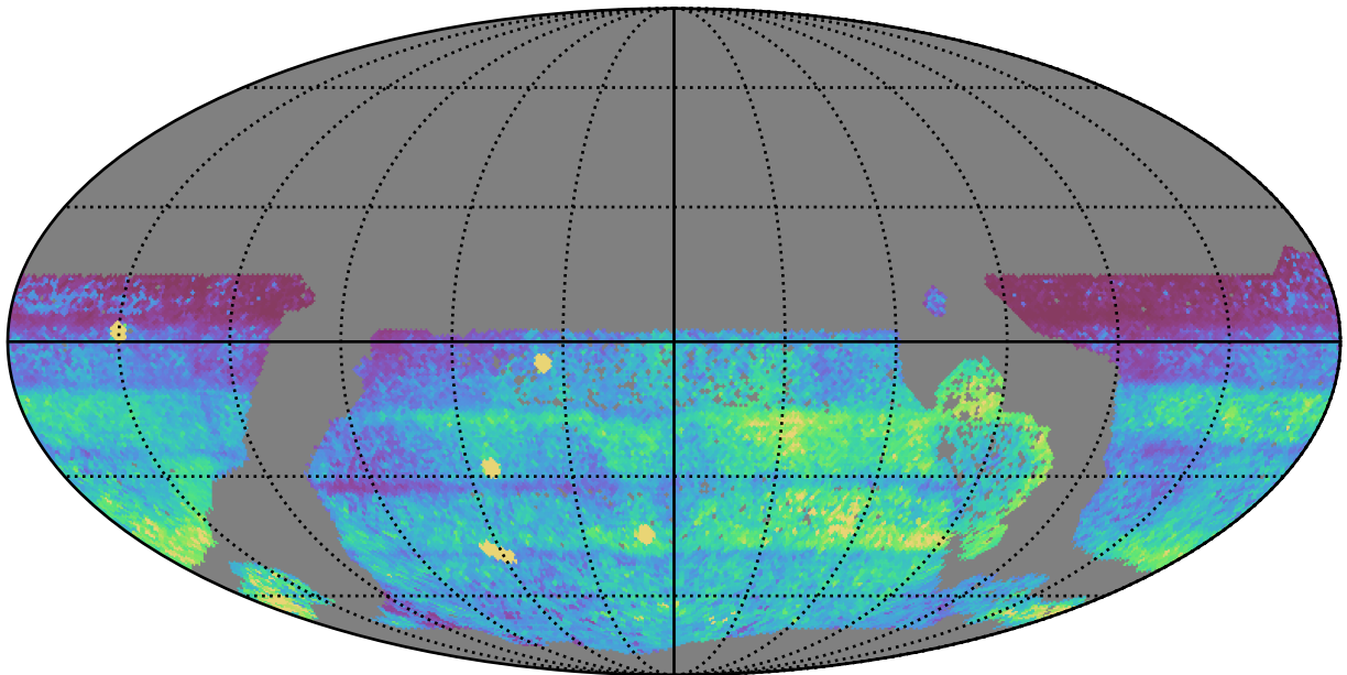
too_elab_r32_d3_giz_v3.4_10yrs WFD all bands: 75th Percentile Intranight Timespan
