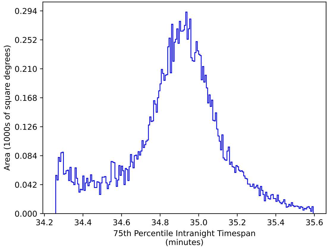
too_elab_r32_d3_giz_v3.4_10yrs WFD all bands: 75th Percentile Intranight Timespan
