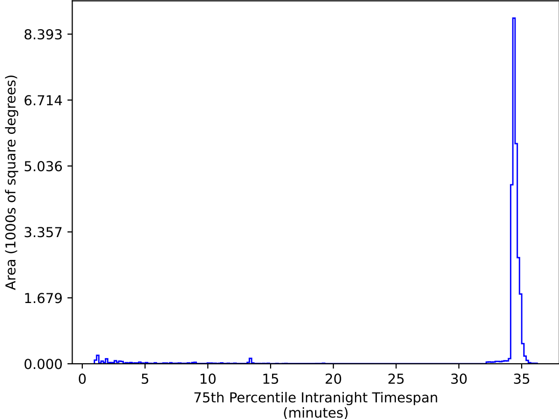
too_elab_r32_d3_giz_v3.4_10yrs All sky zy bands: 75th Percentile Intranight Timespan
