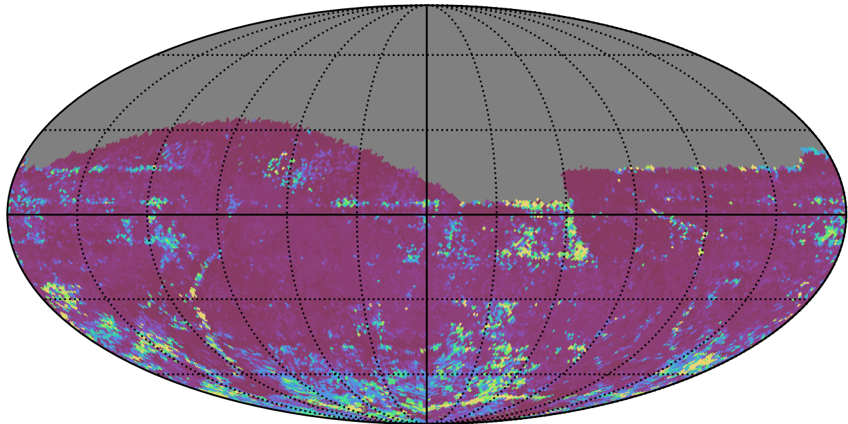
too_elab_r32_d3_giz_v3.4_10yrs All sky z band: 75th Percentile Intranight Timespan
