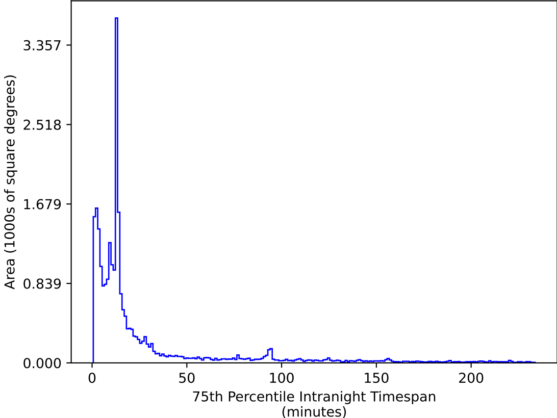
too_elab_r32_d3_giz_v3.4_10yrs All sky z band: 75th Percentile Intranight Timespan
