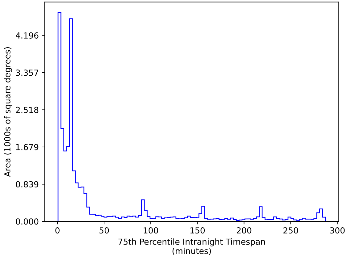
too_elab_r32_d3_giz_v3.4_10yrs All sky r band: 75th Percentile Intranight Timespan
