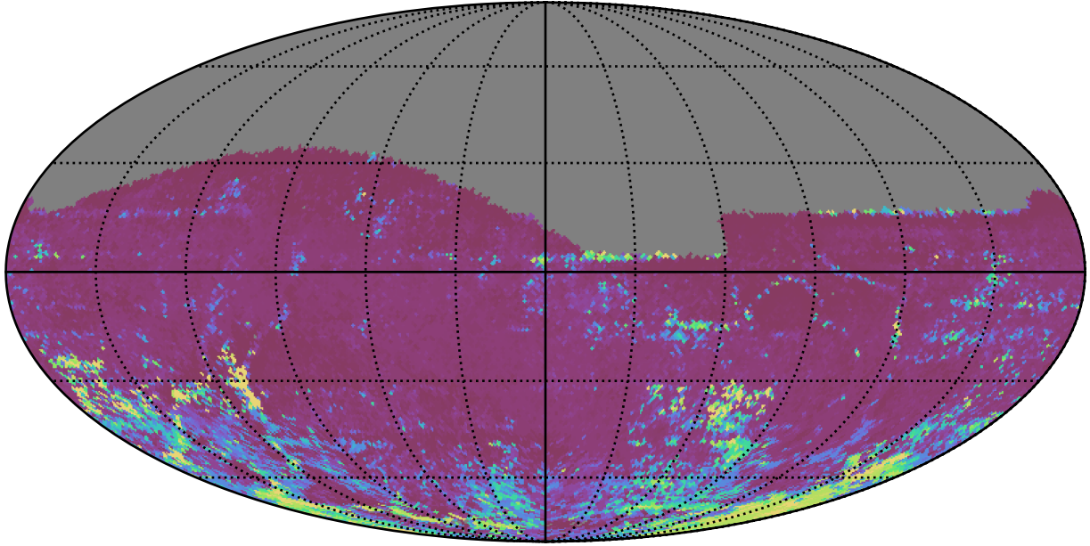
too_elab_r32_d3_giz_v3.4_10yrs All sky i band: 75th Percentile Intranight Timespan
