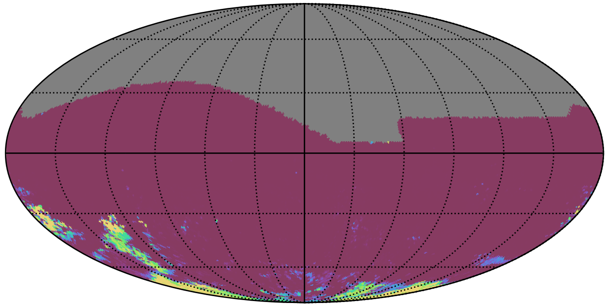
too_elab_r32_d3_giz_v3.4_10yrs All sky gr bands: 75th Percentile Intranight Timespan
