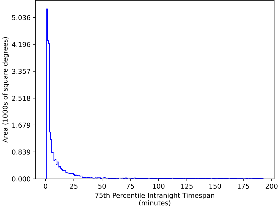
too_elab_r32_d3_giz_v3.4_10yrs All sky g band: 75th Percentile Intranight Timespan
