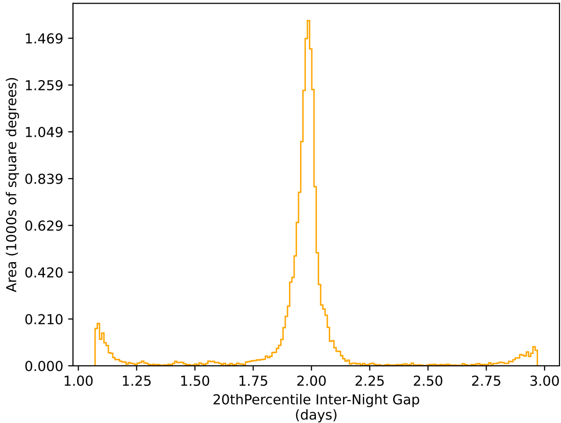
too_elab_r32_d3_giz_v3.4_10yrs WFD r band: 20thPercentile Inter-Night Gap
