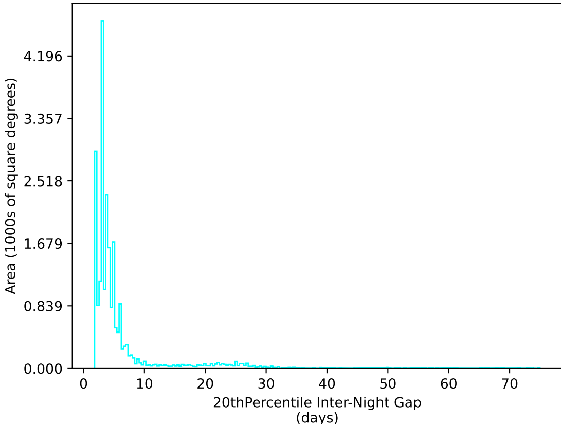
too_elab_r32_d3_giz_v3.4_10yrs All sky u band: 20thPercentile Inter-Night Gap
